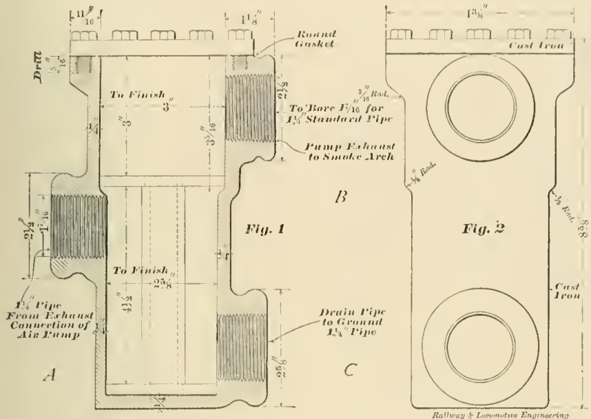
AUTOMATIC AIR-PUMP DRAIN, SECTIONAL AND OUTSIDE VIEW OF VALVE CASE.
